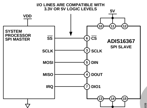
Figure 9. Electrical Connection Diagram
