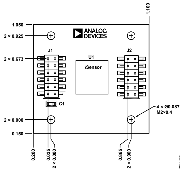
Figure 31. PCB Assembly View and Dimensions
