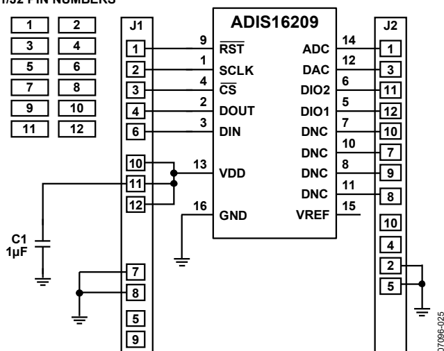
Figure 30. Electrical Schematic
