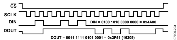
Figure 23. SPI Signal Pattern, Repeating Read of the PROD_ID Register
