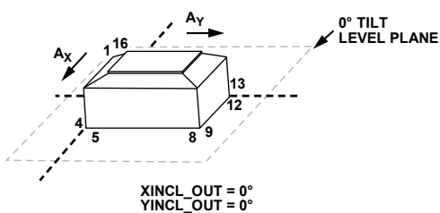
Figure 27. Accelerometer Polarity
