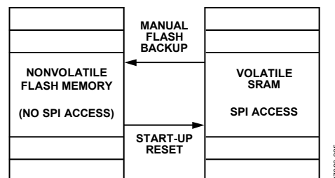
Figure 25. SRAM and Flash Memory Diagram
