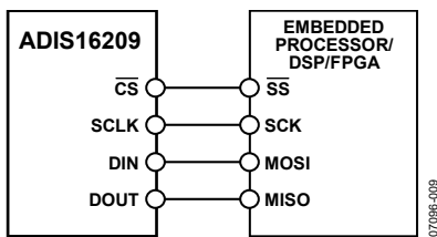
Figure 21. Electrical Connection Diagram
