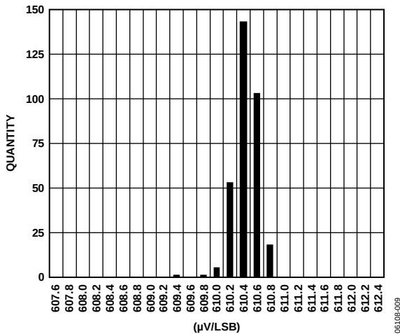
Figure 9. ADC Gain Distribution at 25°C/3.3 V
