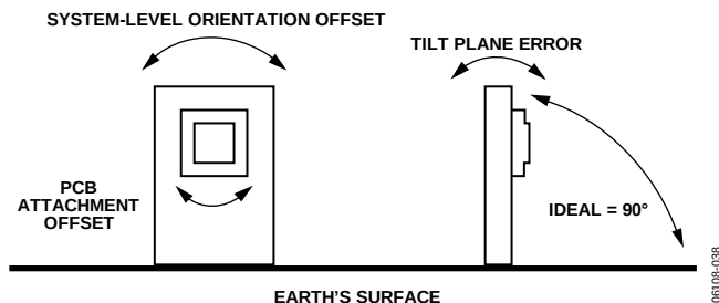
Figure 24. ADIS16203 System-Level Orientation
