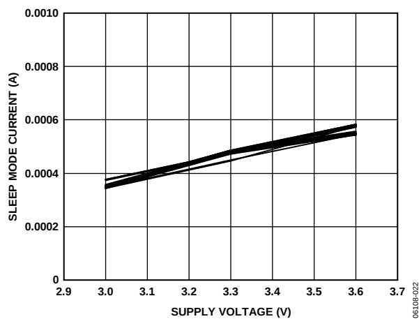
Figure 22. Sleep Mode Current vs. Supply Voltage at 25°C
