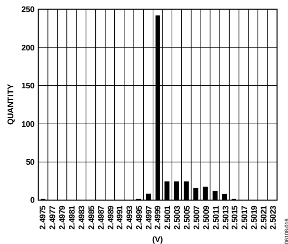
Figure 16. VREF Distribution at 25°C/3.3 V
