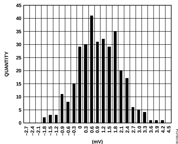
Figure 14. DAC Offset Distribution at 25°C/3.3 V
