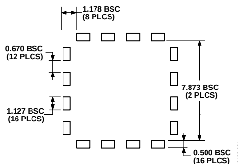
Figure 33. Example Pad Layout
