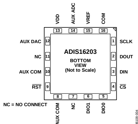
Figure 4. Pin Configuration
