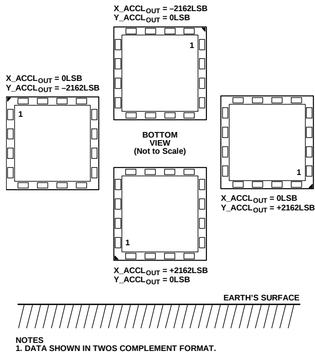
Figure 36. Output Response vs. Orientation
