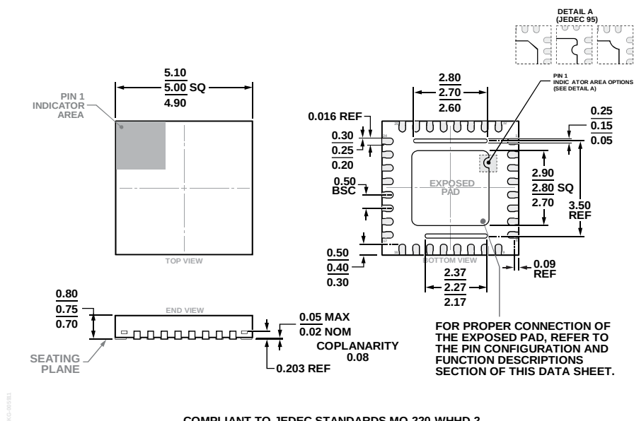
COMPLIANT TO JEDEC STANDARDS MO-220-WHHD-2 Figure 40. 32-Lead Lead Frame Chip Scale Package [LFCSP] 5 mm × 5 mm Body and 0.75 mm Package Height (CP-32-31) Dimensions shown in millimeters
