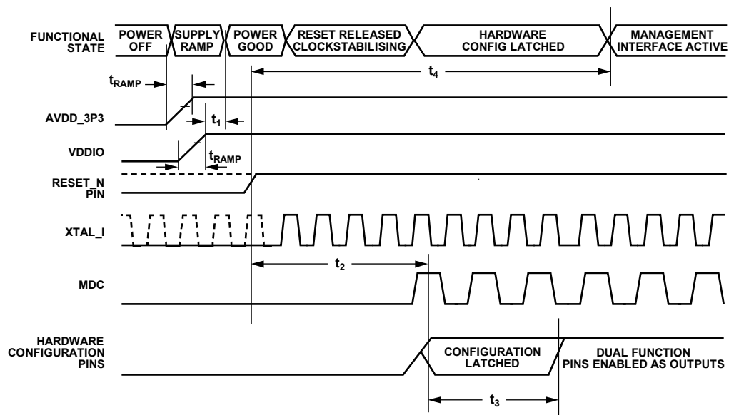
Figure 2. Power-Up Timing
