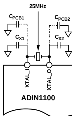
Figure 13. Crystal Oscillator Connection
