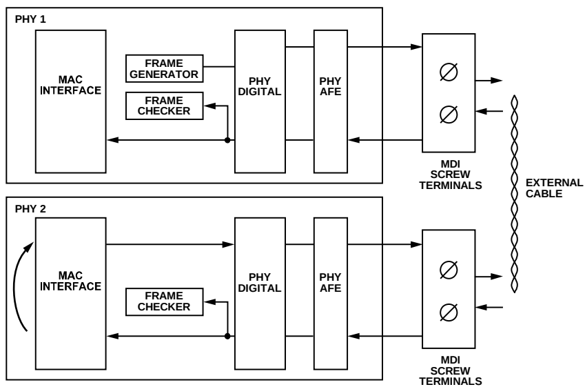
Figure 9. Remote Loopback used across Two PHYs for Self Check Purposes
