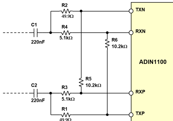
Figure 7. Recommended hybrid for the ADIN1100.
