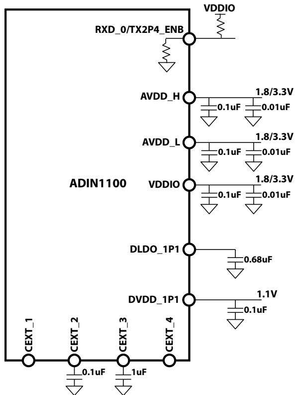
Figure 10. Supplies and capacitors for forced 1V pk-pk transmit mode
