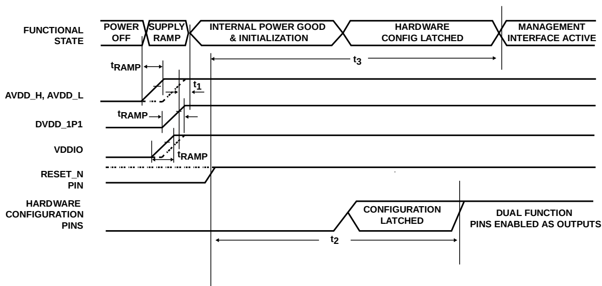
Figure 2. Power-Up Timing
