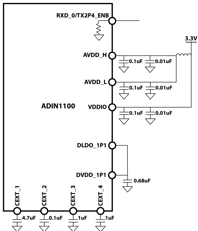
Figure 12. Supplies and capacitors for single supply 2.4 V pk-pk transmit mode
