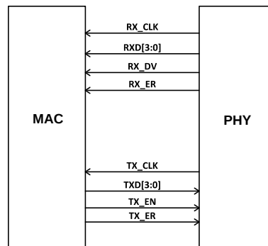
Figure 5. MII MAC-PHY Interface Signals
