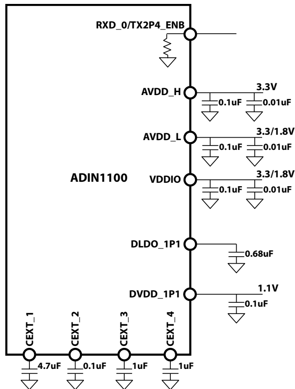
Figure 11. Supplies and capacitors for 2.4/1.0 V pk-pk transmit mode
