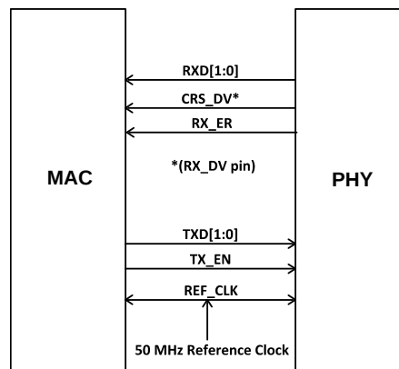
Figure 6. RMII MAC-PHY Interface Signals
