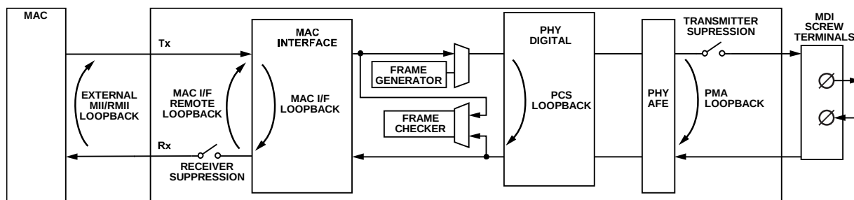
Figure 8. ADIN1100 Loopback Modes
