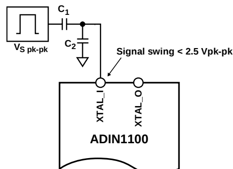
Figure 14. External Clock Connection
