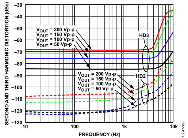
Figure 40. Second Harmonic Distortion (HD2) and Third Harmonic Distortion (HD3) vs. Frequency at Various Output Swings, T_A = 25^\circ\text{C} , A_V = 20 , V_S = \pm 110 V, R_F = 100 k \Omega , R_{LOAD} = 10 k \Omega , R_{ADJ} = 0 \Omega
