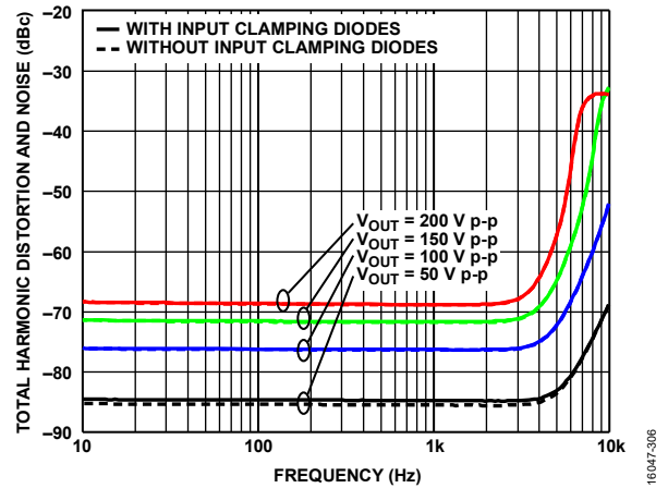
Figure 38. Total Harmonic Distortion and Noise vs. Frequency at Various Large Output Swings, T_A = 25^\circ\text{C} , A_V = 20 , V_S = \pm 110 V, R_F = 100 k \Omega , R_{LOAD} = 10 k \Omega , R_{ADJ} = 0 \Omega
