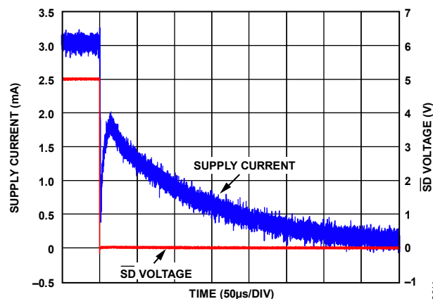
Figure 54. \overline{\text{SD}} Pin Response Time, Turning Off
