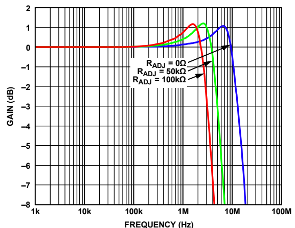
Figure 51. Small Signal Frequency Response at Various R_{ADJ} , T_A = 25^\circ\text{C} , A_V = 1 , V_S = \pm 110 V, V_{OUT} = 100 mV p-p, R_F = 0 \Omega , R_{LOAD} = 10 k \Omega
