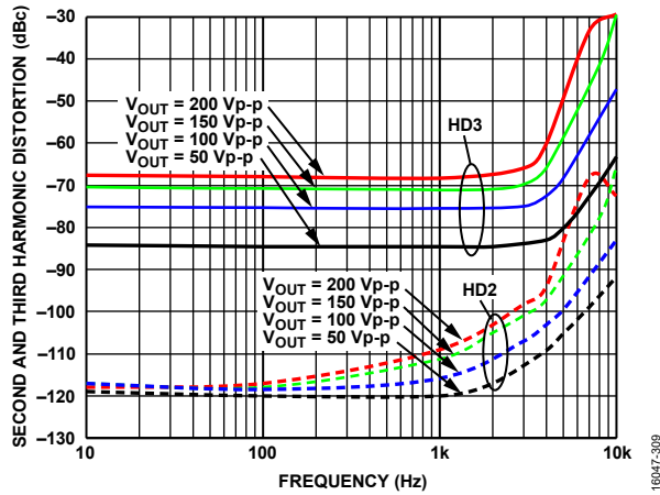
Figure 41. Second Harmonic Distortion (HD2) and Third Harmonic Distortion (HD3) vs. Frequency at Various Output Swings, T_A = 25^\circ\text{C} , A_v = 40 , V_S = \pm 110\text{ V} , R_F = 100\text{ k}\Omega , R_{LOAD} = 10\text{ k}\Omega , R_{ADJ} = 0\text{ }\Omega
