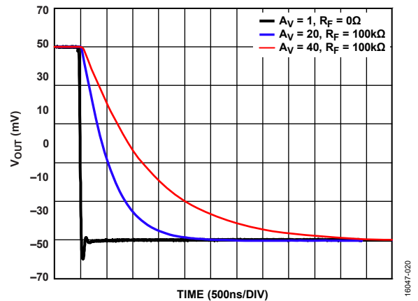
Figure 27. Small Signal Pulse Response at Various Gains, Falling Edge, T_A = 25^\circ\text{C} , V_S = \pm 110\text{ V} , V_{\text{OUT}} = 100\text{ mV p-p} , R_{\text{LOAD}} = 10\text{ k}\Omega , R_{\text{ADJ}} = 0\text{ }\Omega
