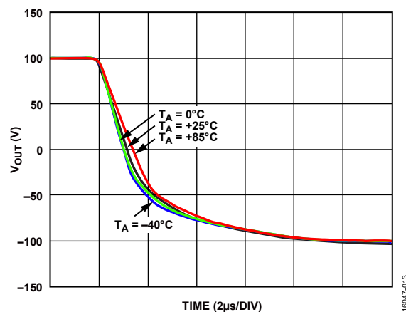
Figure 20. Large Signal Pulse Response at Various T_A , Falling Edge, A_V = 40 , V_S = \pm 110\text{ V} , V_{OUT} = 200\text{ V p-p} , R_F = 100\text{ k}\Omega , R_{LOAD} = 10\text{ k}\Omega , R_{ADJ} = 0\text{ }\Omega
