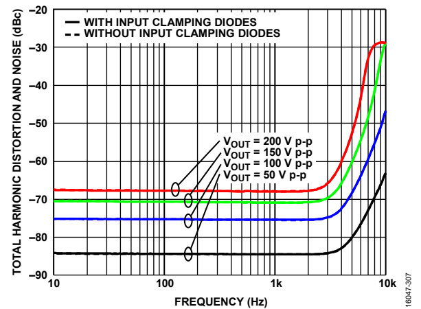
Figure 39. Total Harmonic Distortion and Noise vs. Frequency at Various Large Output Swings, T_A = 25^\circ\text{C} , A_V = 40 , V_S = \pm 110 V, R_F = 100 k \Omega , R_{LOAD} = 10 k \Omega , R_{ADJ} = 0 \Omega
