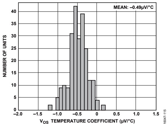
Figure 7. Input Offset Voltage Drift Distribution, T_A = 25^\circ\text{C} , V_S = \pm 110\text{ V} , V_{CM} = 0\text{ V} , \Delta T_J = 60^\circ\text{C} , R_{ADJ} = 0\ \Omega
