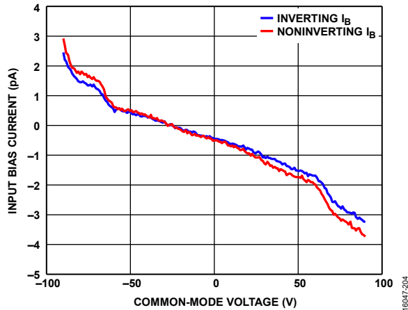
Figure 30. Input Bias Current vs. Common-Mode Voltage, T_A = 25^\circ\text{C} , V_S = \pm 110\text{ V} , R_{ADJ} = 0\ \Omega
