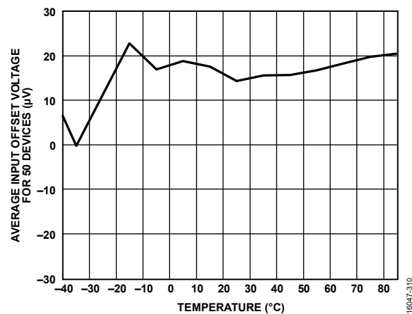
Figure 10. Average Input Offset Voltage for 50 Devices vs. Temperature, V_S = \pm 110\text{ V}
