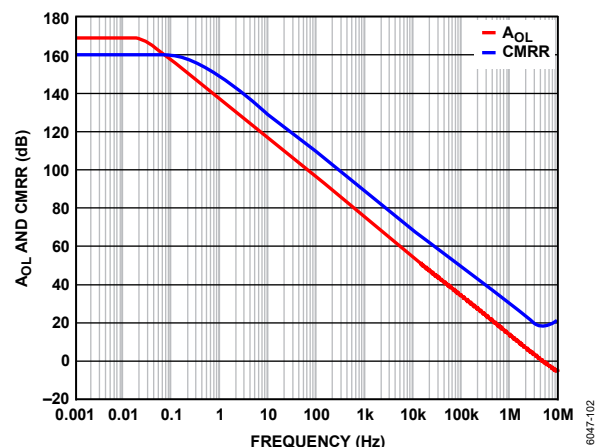
Figure 2. ADHV4702-1 Precision Performance
