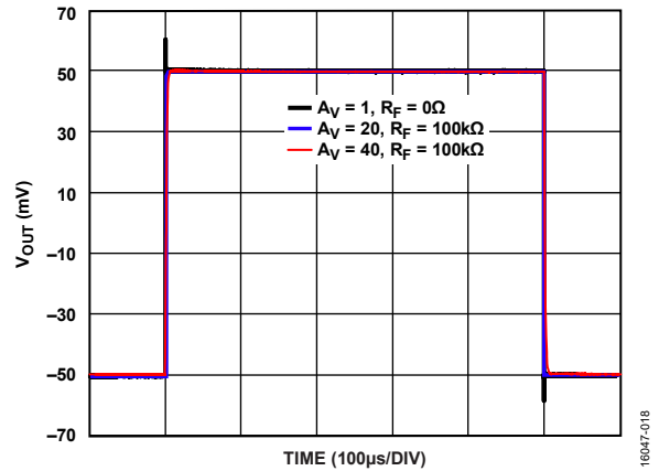
Figure 26. Small Signal Pulse Response at Various Gains, T_A = 25^\circ\text{C} , V_S = 110\text{ V} , V_{\text{OUT}} = 100\text{ mV p-p} , R_{\text{LOAD}} = 10\text{ k}\Omega , R_{\text{ADJ}} = 0\text{ }\Omega
