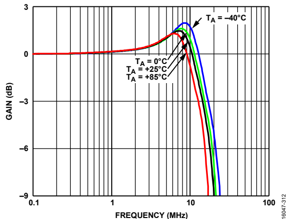
Figure 25. Small Signal Frequency Response at Various T_A , A_V = 1 , V_S = \pm 110\text{ V} , V_{\text{OUT}} = 100\text{ mV p-p} , R_L = 10\text{ k}\Omega , R_{\text{ADJ}} = 0\text{ }\Omega
