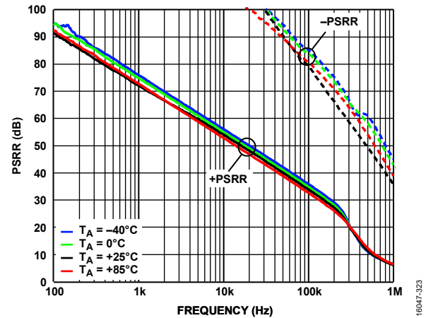
Figure 43. PSRR vs. Frequency at Various T_A , V_S = \pm 110\text{ V} , R_{LOAD} = 10\text{ k}\Omega , R_{ADJ} = 0\text{ }\Omega
