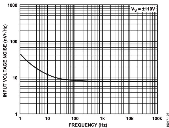
Figure 31. Input Voltage Noise vs. Frequency, T_A = 25^\circ\text{C} , V_S = \pm 110 , R_{ADJ} = 0\ \Omega
