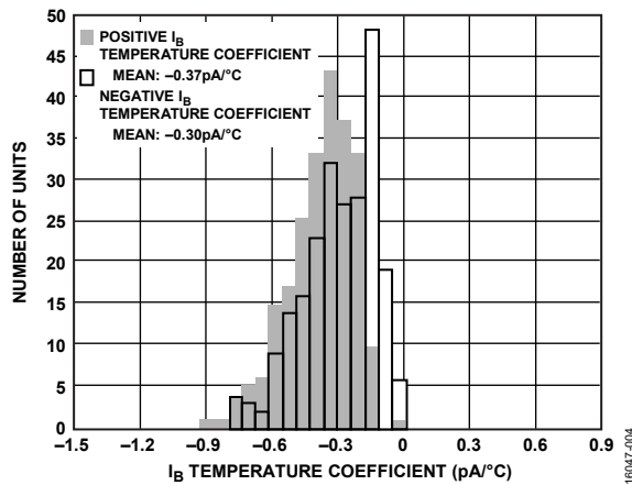
Figure 5. Positive and Negative Input Bias ( I_B ) Current Drift Distribution, T_A = 25^\circ\text{C} , V_S = \pm 110\text{ V} , V_{CM} = 0\text{ V} , \Delta T_A = 60^\circ\text{C} , R_{ADJ} = 0\ \Omega
