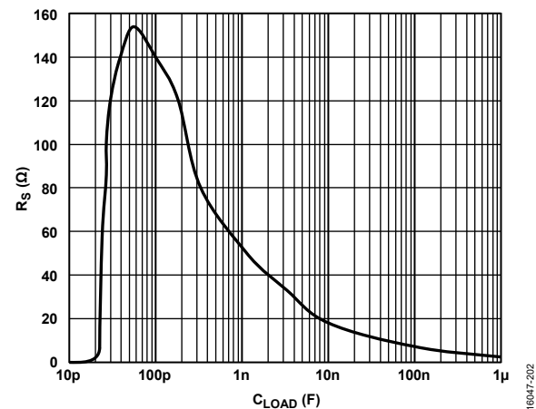
Figure 58. R_S vs. C_{LOAD} for Maximum 2 dB Peaking for Circuit from Figure 57, T_A = 25^\circ\text{C} , A_V = 1 , V_S = \pm 110\text{ V} , V_{OUT} = 100\text{ mV p-p} , R_F = 0\ \Omega , R_{ADJ} = 0\ \Omega
