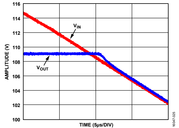
Figure 44. Output Overdrive Recovery, V_S = \pm 110\text{ V} , A_v = 40 , R_{LOAD} = 10\text{ k}\Omega , R_{ADJ} = 0\text{ }\Omega
