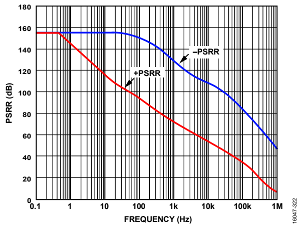
Figure 42. PSRR vs. Frequency, T_A = 25^\circ\text{C} , V_S = \pm 110\text{ V} , R_{LOAD} = 10\text{ k}\Omega , R_{ADJ} = 0\text{ }\Omega
