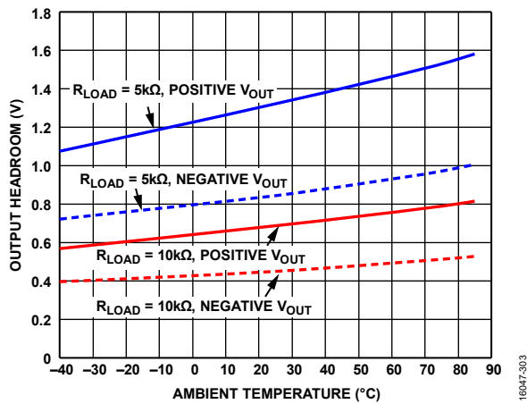
Figure 36. Output Headroom vs. Ambient Temperature at Various R_{LOAD} , V_S = \pm 110 V, R_{ADJ} = 0 \Omega
