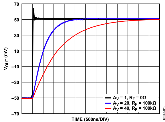
Figure 24. Small Signal Pulse Response at Various Gains, Rising Edge, T_A = 25^\circ\text{C} , V_S = \pm 110\text{ V} , V_{\text{OUT}} = 100\text{ mV p-p} , R_{\text{LOAD}} = 10\text{ k}\Omega , R_{\text{ADJ}} = 0\text{ }\Omega
