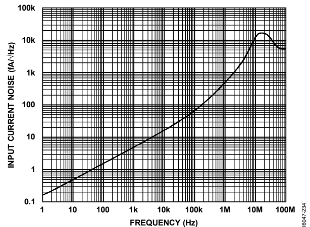
Figure 34. Input Current Noise vs. Frequency
