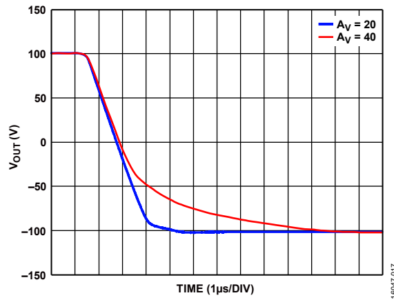
Figure 21. Large Signal Pulse Response at Various Gains, Falling Edge, T_A = 25^\circ\text{C} , V_S = \pm 110\text{ V} , V_{OUT} = 200\text{ V p-p} , R_F = 100\text{ k}\Omega , R_{LOAD} = 10\text{ k}\Omega , R_{ADJ} = 0\text{ }\Omega
