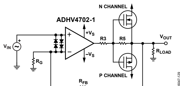
Figure 64. High Current Output Driver Schematic
