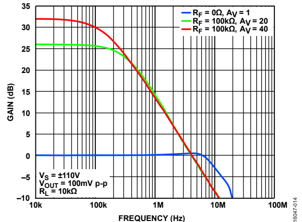
Figure 28. Small Signal Frequency Response at Various Gains, T_A = 25^\circ\text{C} , V_S = \pm 110\text{ V} , V_{\text{OUT}} = 100\text{ mV p-p} , R_L = 10\text{ k}\Omega , R_{\text{ADJ}} = 0\text{ }\Omega
