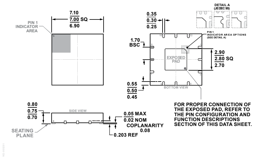
Figure 66. 12-Lead Lead Frame Chip Scale Package [LFCSP] 7 mm x 7 mm Body and 0.75 mm Package Height (CP-12-8)
