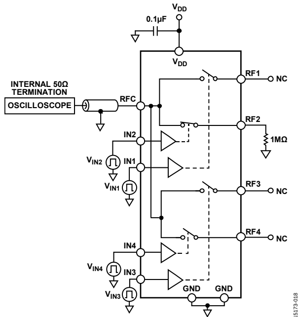
Figure 36. Video Feedthrough
