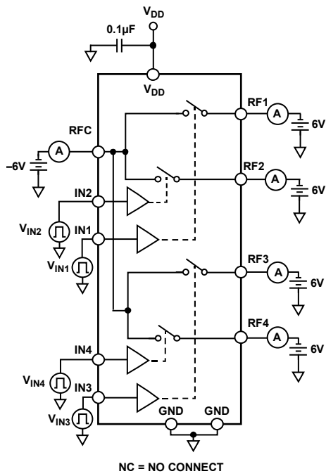
Figure 41. Off Leakage
