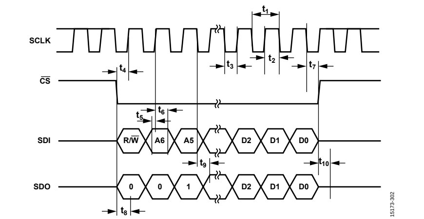
Figure 2. Addressable Mode Timing Diagram
