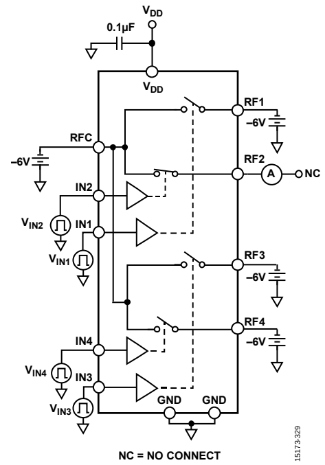
Figure 43. On Leakage
