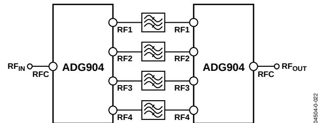
Figure 28. Filter Selection
