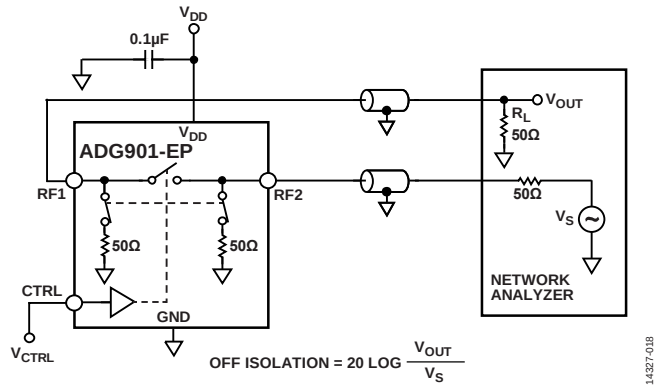
Figure 18. Off Isolation
