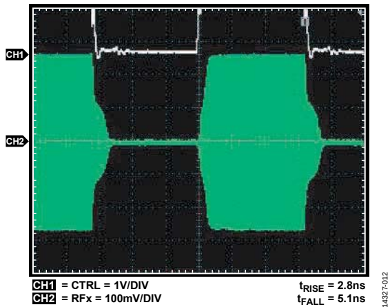
Figure 12. Switch Timing
