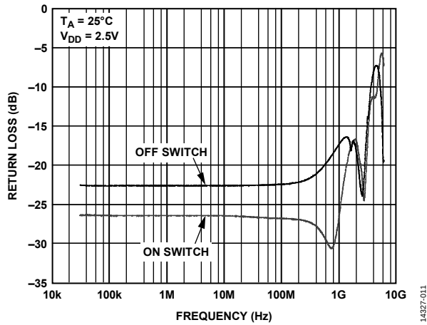
Figure 11. Return Loss vs. Frequency ( S_{11} )
