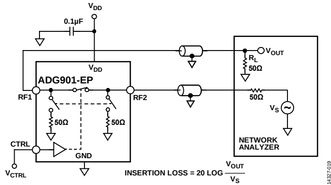
Figure 19. Insertion Loss
