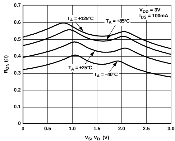
Figure 8. On Resistance vs. V_D ( V_S ) for Different Temperatures, V_{DD} = 3 V
