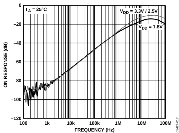
Figure 17. AC PSRR
