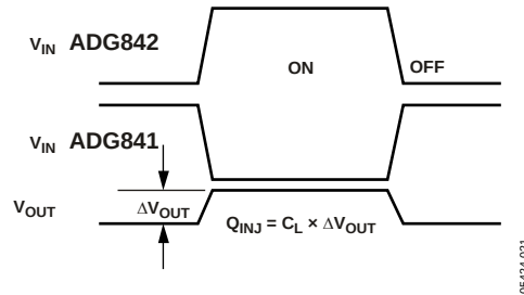
Figure 22. Charge Injection
