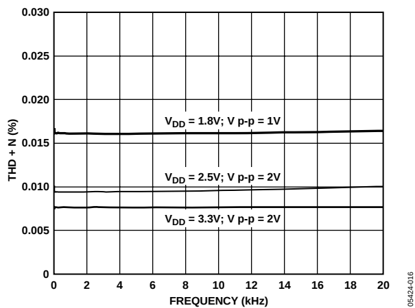
Figure 16. Total Harmonic Distortion + Noise
