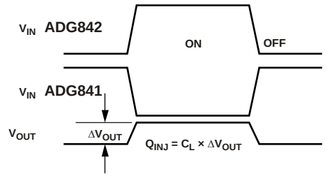
Figure 22. Charge Injection
