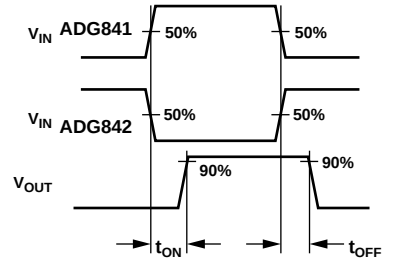
Figure 21. Switching Times, t_{ON} , t_{OFF}
