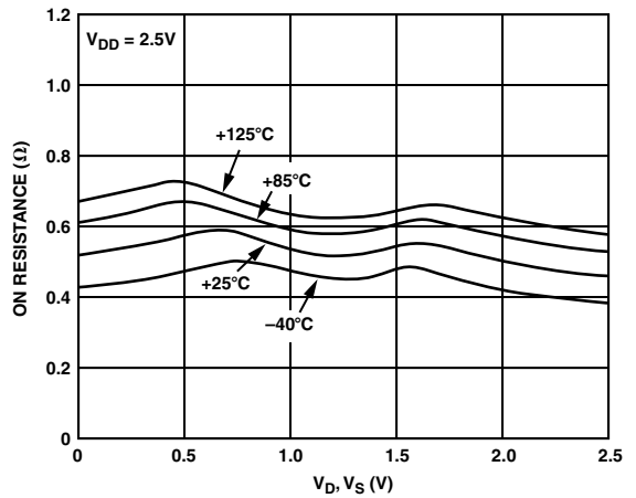
TPC 5. On Resistance vs. V_D ( V_S ) for Different Temperature, 2.5\text{V}
