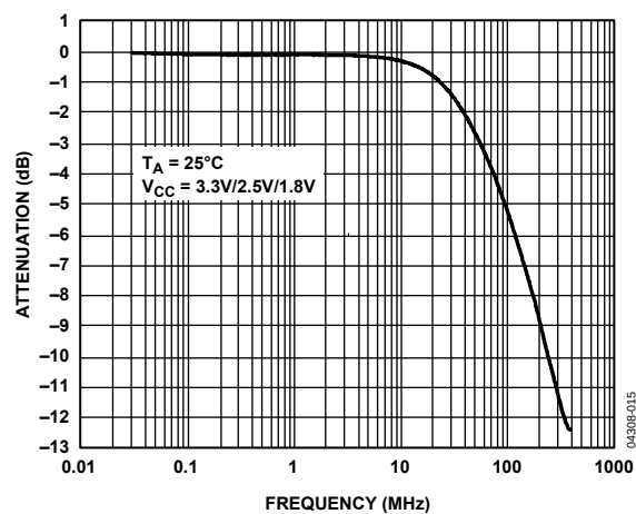
Figure 15. Bandwidth
