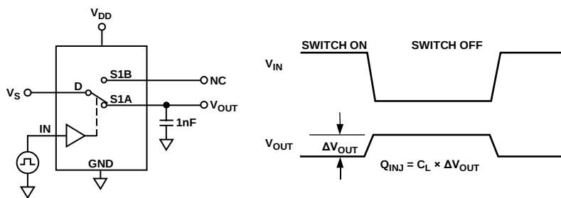
Figure 24. Charge Injection
