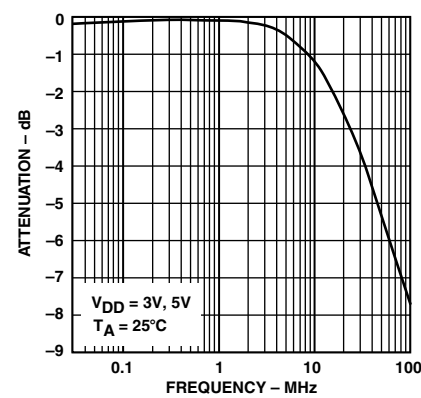
TPC 9. On Response vs. Frequency
