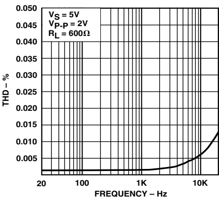
TPC 12. THD
