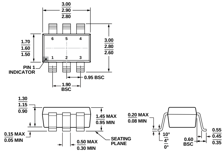
Figure 25. 6-Lead Small Outline Transistor Package [SOT-23] (RJ-6) Dimensions shown in millimeters
