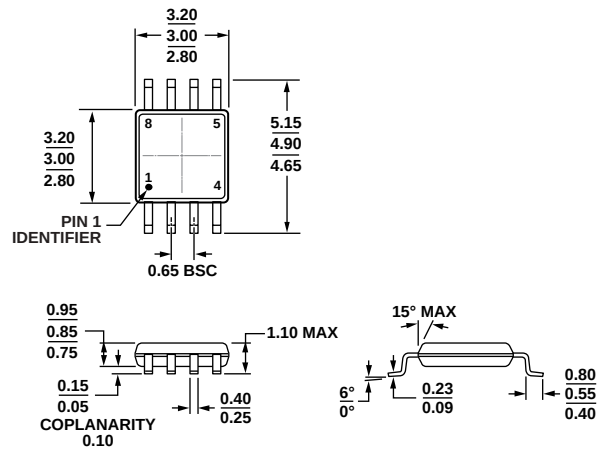
Figure 26. 8-Lead mini Small Outline Package [MSOP] (RM-8) Dimensions shown in millimeters
