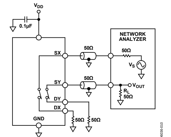
Figure 23. Channel-to-Channel Crosstalk
