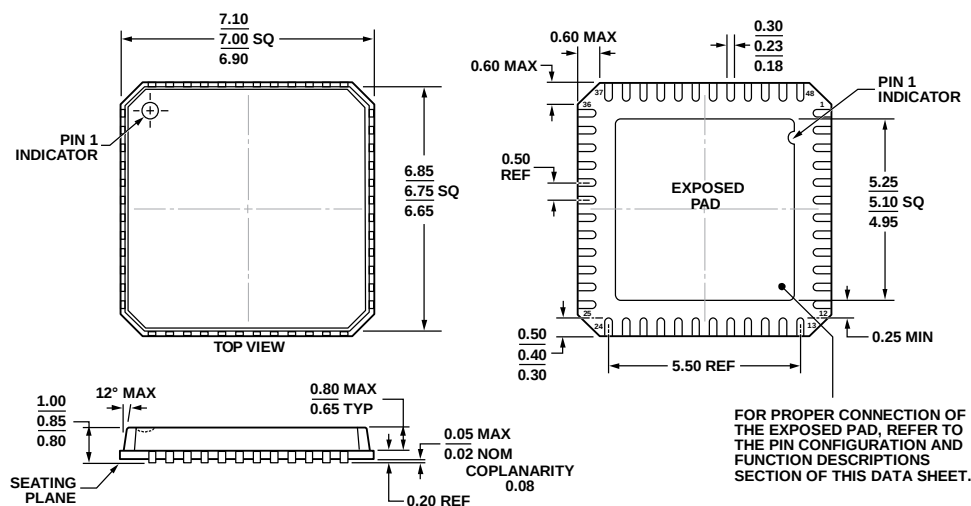
Figure 32. 48-Lead Frame Chip Scale Package [LFCSP_VQ] 7 mm × 7 mm Body, Very Thin Quad (CP-48-1)
