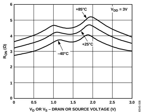
Figure 6. On Resistance as a Function of a V_D ( V_S ) for Different Temperatures, V_{DD} = 3\text{V}
