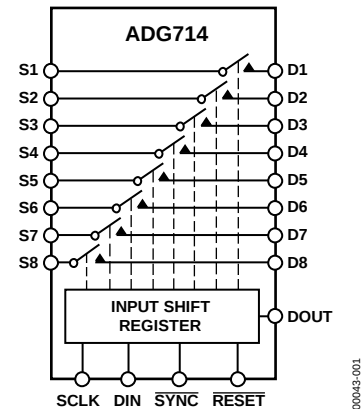
Figure 1. ADG714 Functional Block Diagram
