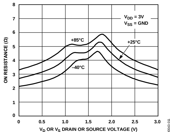
Figure 11. On Resistance as a Function of V_D ( V_S ) for Different Temperatures, V_{DD} = 3\text{V}
