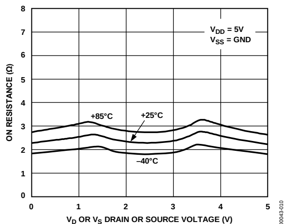
Figure 10. On Resistance as a Function of V_D ( V_S ) for Different Temperatures, V_{DD} = 5\text{V}
