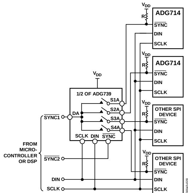
Figure 29. Addressing Multiple ADG714 Devices Using an ADG739
