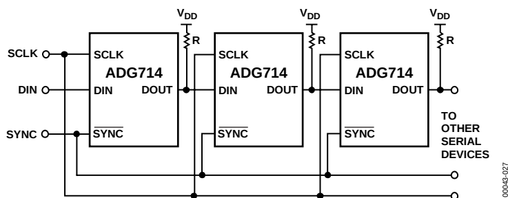
Figure 28. Multiple ADG714 Devices in a Daisy-Chained Configuration
