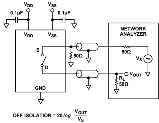
Figure 21. Off Isolation
