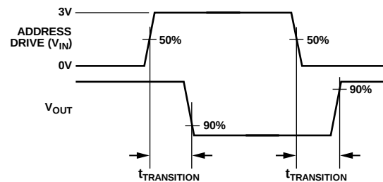
Figure 24. Transition Time, t_{\text{TRANSITION}}
