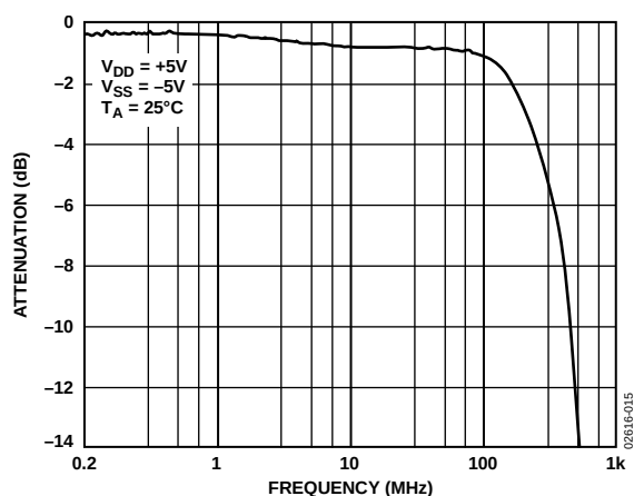
Figure 13. Bandwidth vs. Frequency
