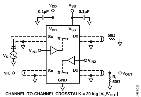
Figure 21. Channel-to-Channel Crosstalk
