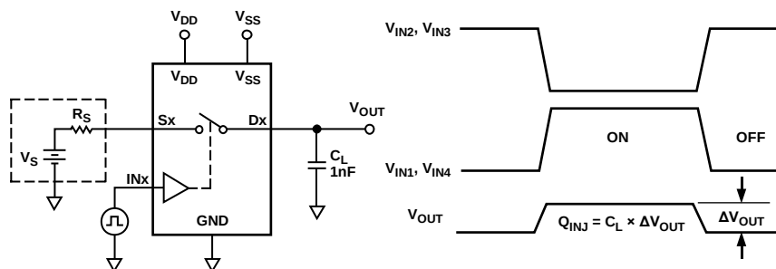
Figure 19. Charge Injection
