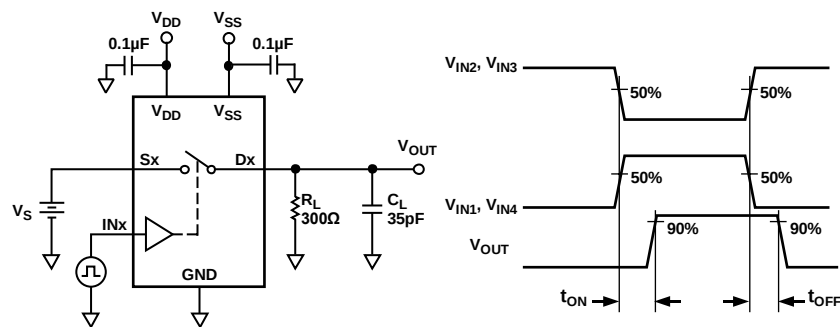
Figure 17. Switching Times
