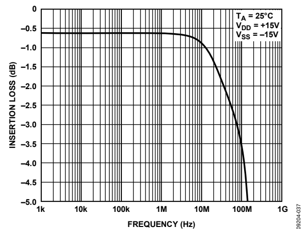
Figure 22. Bandwidth
