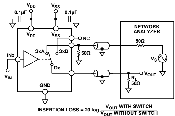
Figure 31. Bandwidth
