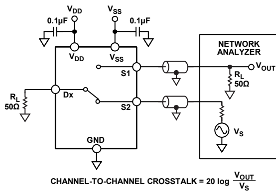
Figure 36. Channel-to-Channel Crosstalk
