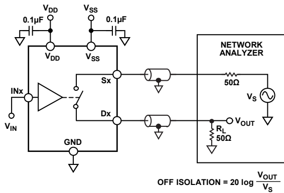
Figure 35. Off Isolation
