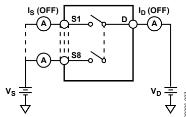
Figure 29. Off Leakage
