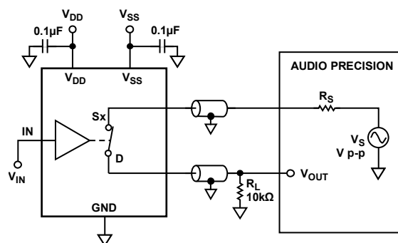
Figure 30. THD + Noise Figure
