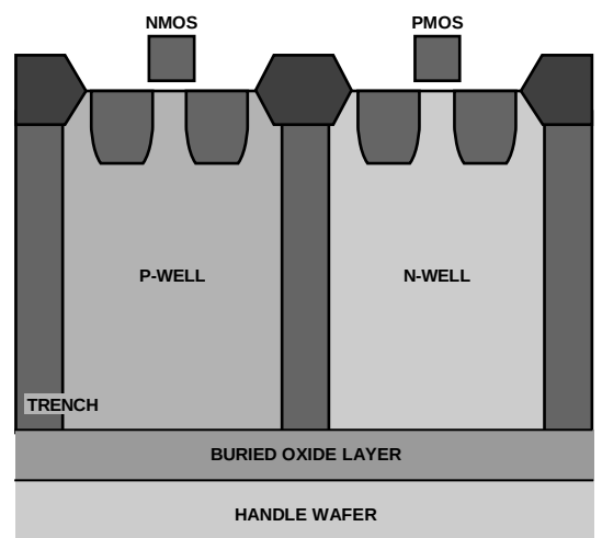
Figure 36. Trench Isolation
