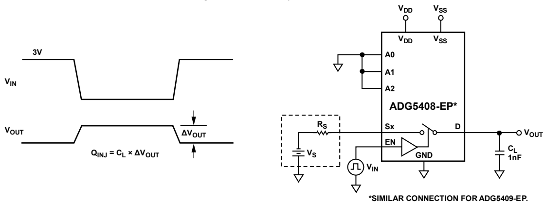
Figure 33. Charge Injection
