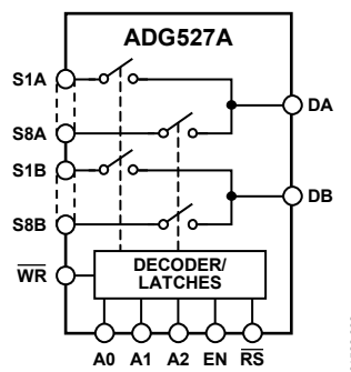
Figure 2. ADG527A
