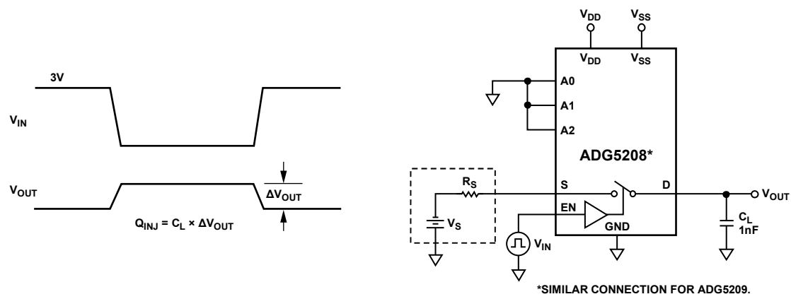
Figure 36. Charge Injection
