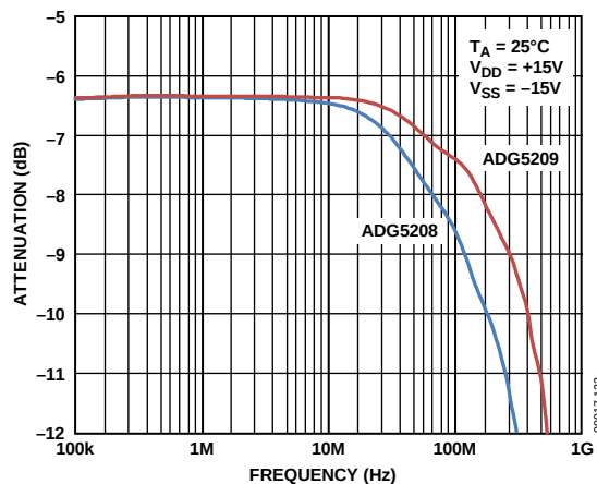
Figure 21. Bandwidth
