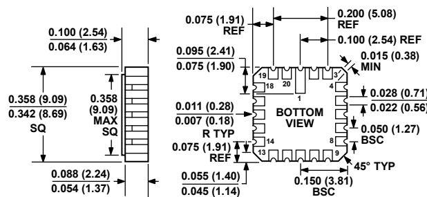
Figure 28. 20-Terminal Ceramic Leadless Chip Carrier [LCC] (E-20-1)
