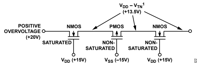
Figure 22. Positive Overvoltage on the Channel Protector
