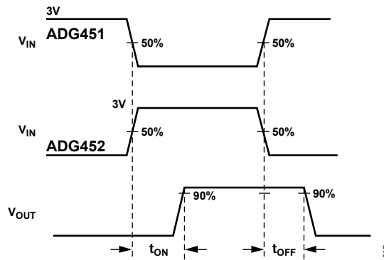
Figure 19. Switching Times
