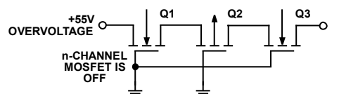
Figure 31. +55\text{ V} Overvoltage with Power Off
