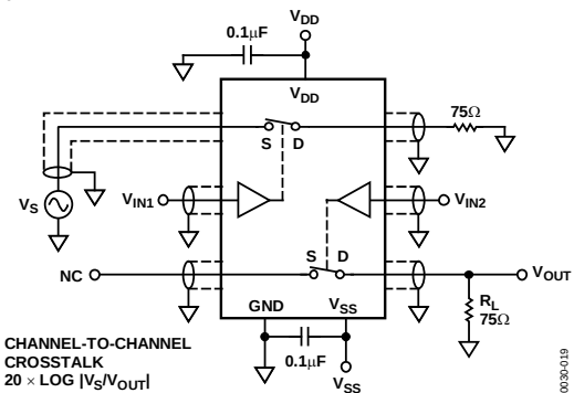
Figure 19. Channel-to Channel Crosstalk
