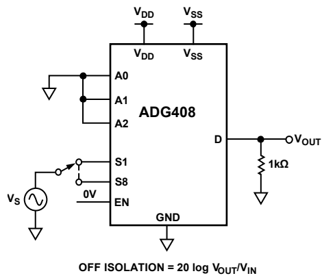
Figure 26. Off Isolation
