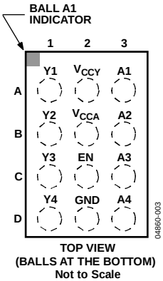
Figure 4. 12-Ball WLCSP Pin Configuration
