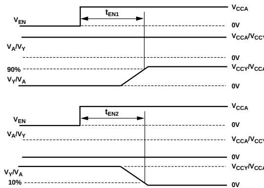
Figure 36. Enable Time
