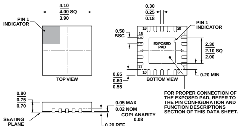
Figure 44. 20-Lead Lead Frame Chip Scale Package [LFCSP] 4 mm × 4 mm Body and 0.75 mm Package Height (CP-20-6)
