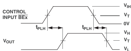
Figure 2. Propagation Delay
