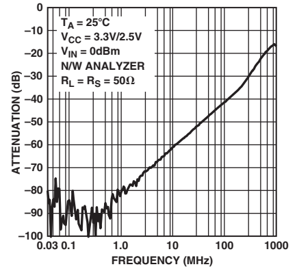
TPC 12. Crosstalk vs. Frequency
