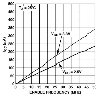
TPC 7. I_{CC} vs. Enable Frequency
