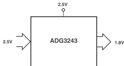
Figure 7. 2.5 V to 1.8 V Voltage Translation
