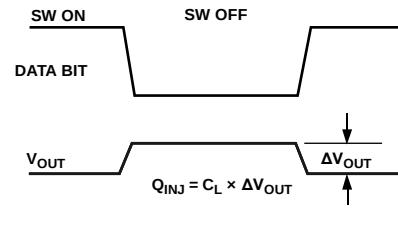
Figure 29. Charge Injection
