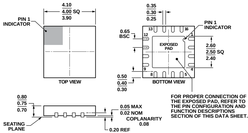
Figure 35. 16-Lead Lead Frame Chip Scale Package [LFCSP] 4 mm × 4 mm Body and 0.75 mm Package Height (CP-16-26)
