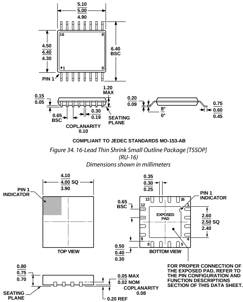
Figure 35. 16-Lead Lead Frame Chip Scale Package [LFCSP] 4 mm × 4 mm Body and 0.75 mm Package Height (CP-16-26)
