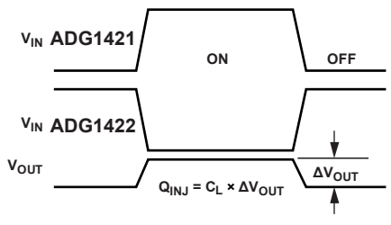
Figure 28. Charge Injection
