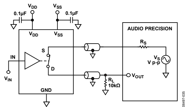
Figure 29. THD + Noise
