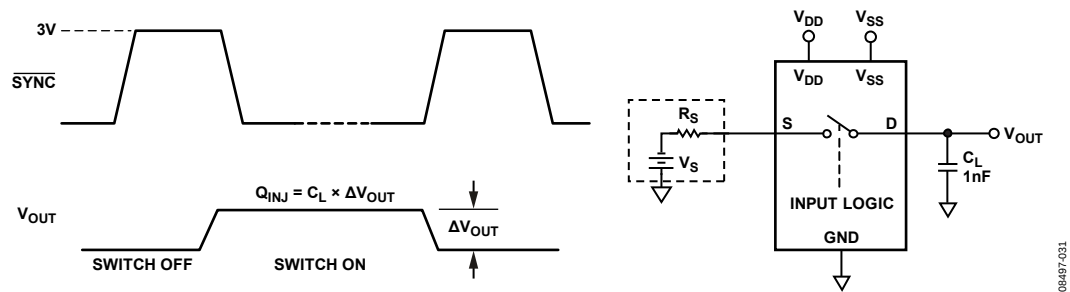
Figure 31. Charge Injection
