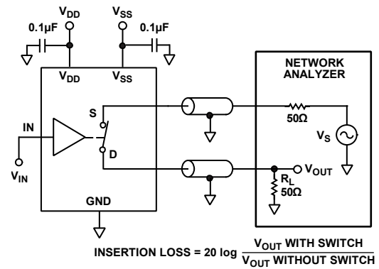
Figure 28. Insertion Loss
