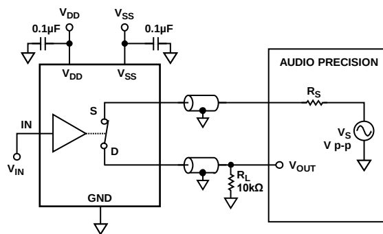
Figure 36. THD + N
