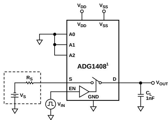
Figure 32. Charge Injection
