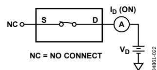
Figure 28. On Leakage
