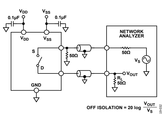
Figure 34. Off Isolation
