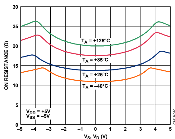
Figure 11. On Resistance as a Function of V_D ( V_S ) for Different Temperatures, 5 V Dual Supply
