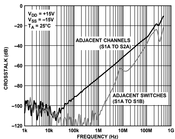
Figure 22. ADG1407 Crosstalk vs. Frequency
