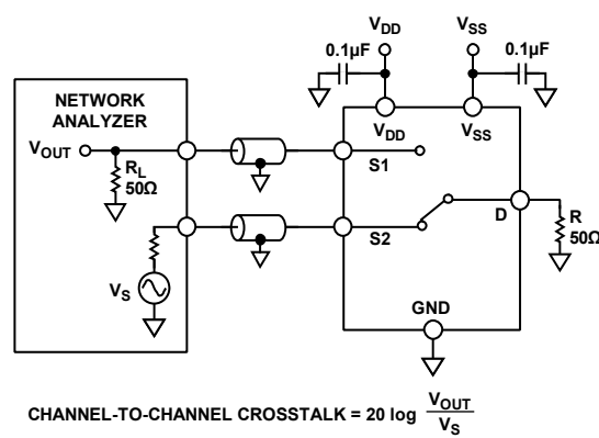
Figure 36. Channel-to-Channel Crosstalk
