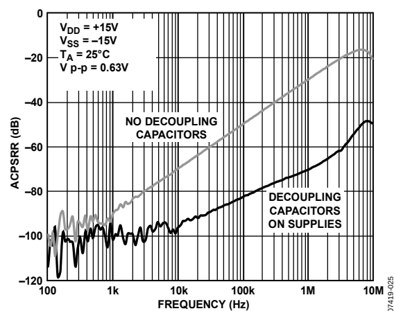
Figure 26. ACPSSRR vs. Frequency
