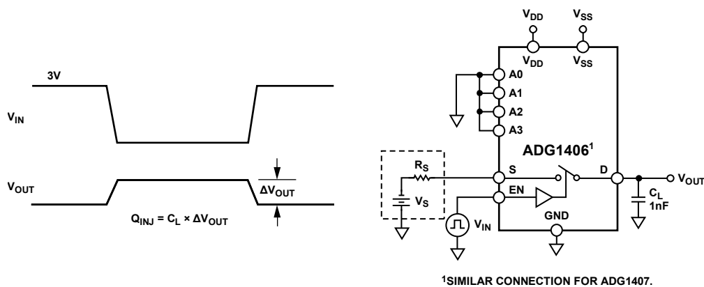
Figure 33. Charge Injection
