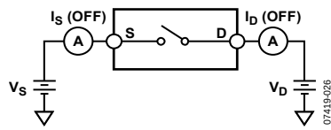
Figure 28. Off Leakage
