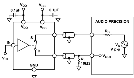
Figure 37. THD + N
