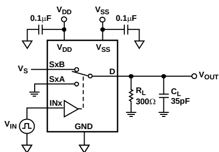
Figure 14. Switching Timing
