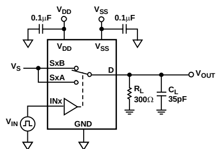
Figure 15. Break-Before-Make Delay
