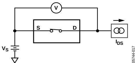
Figure 11. On Resistance
