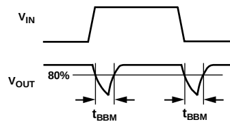
Figure 15. Break-Before-Make Delay
